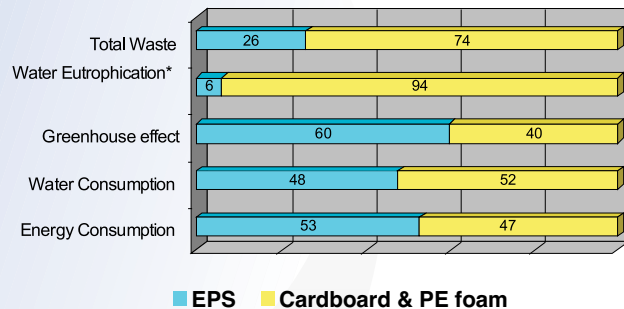
Figure 2: A selection of environmental indicators (reference scenario)
